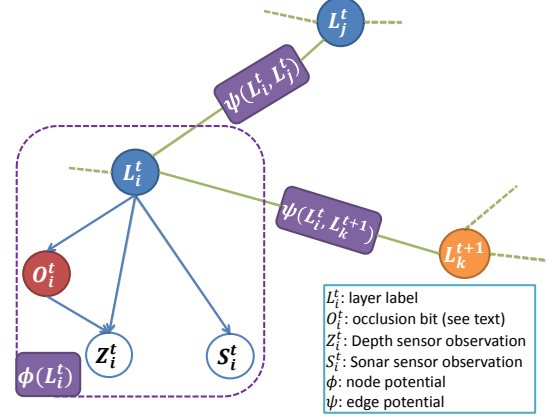
Figure 2. The graphical model shows the conditional dependence structure between random variables and the smoothing term on the right side defines the constraints between neighboring labels while the data term on the left side describes the sensor measurement process.
