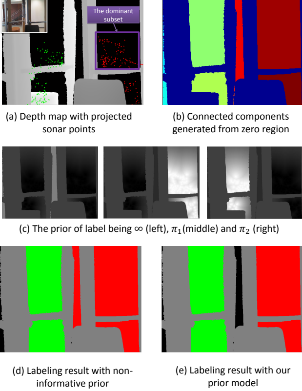
Figure 3. An example demonstrating our prior model. In this example \pi_1 is the surface fitted from the entire red points in (a) and \pi_2 is the surface fitted from the entire green points in (a).
