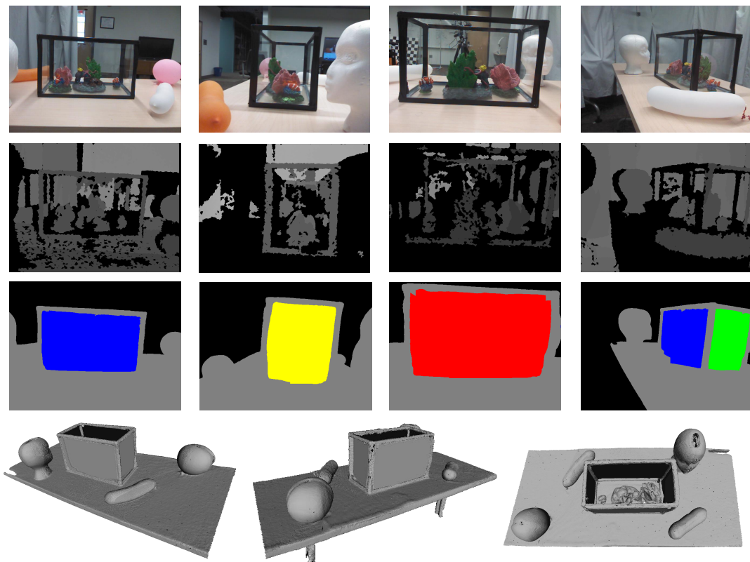
Figure 7. Our results on fish tank scene. We scanned the fish tank separately from four different sides, the third row shows the labeling. The final row shows the final merged result.
