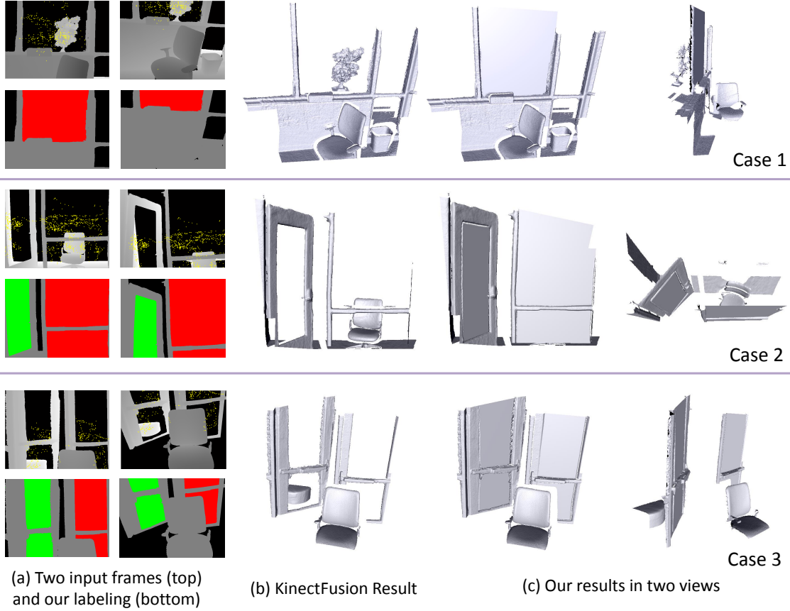
Figure 6. Our results on various real scenes.
