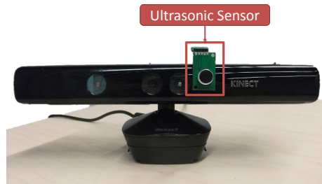
Figure 1. Our modified Kinect camera has an additional ultrasonic range sensor (e.g., a sonar), which can measure distance to any objects, including transparent ones.
