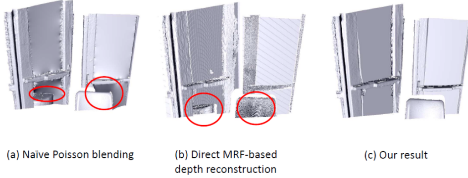
Figure 5. Comparison of our result with two other alternatives. Artifacts produced by these alternatives are highlighted in the red circles.
