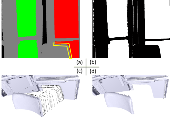
Figure 4. A basic mask for Poisson blending can be obtained from our labeling result in (a). In this case, the mask will contain the red and the green region. To reduce the noises in the object boundary caused by the depth sensor, we extend this mask by dilating the mask for 5 pixels. The boundary along empty space is also included and the resulting mask is shown in (b). (c) and (d), which demonstrates the necessity of adopting the adaptive differential operators during Poisson blending.
