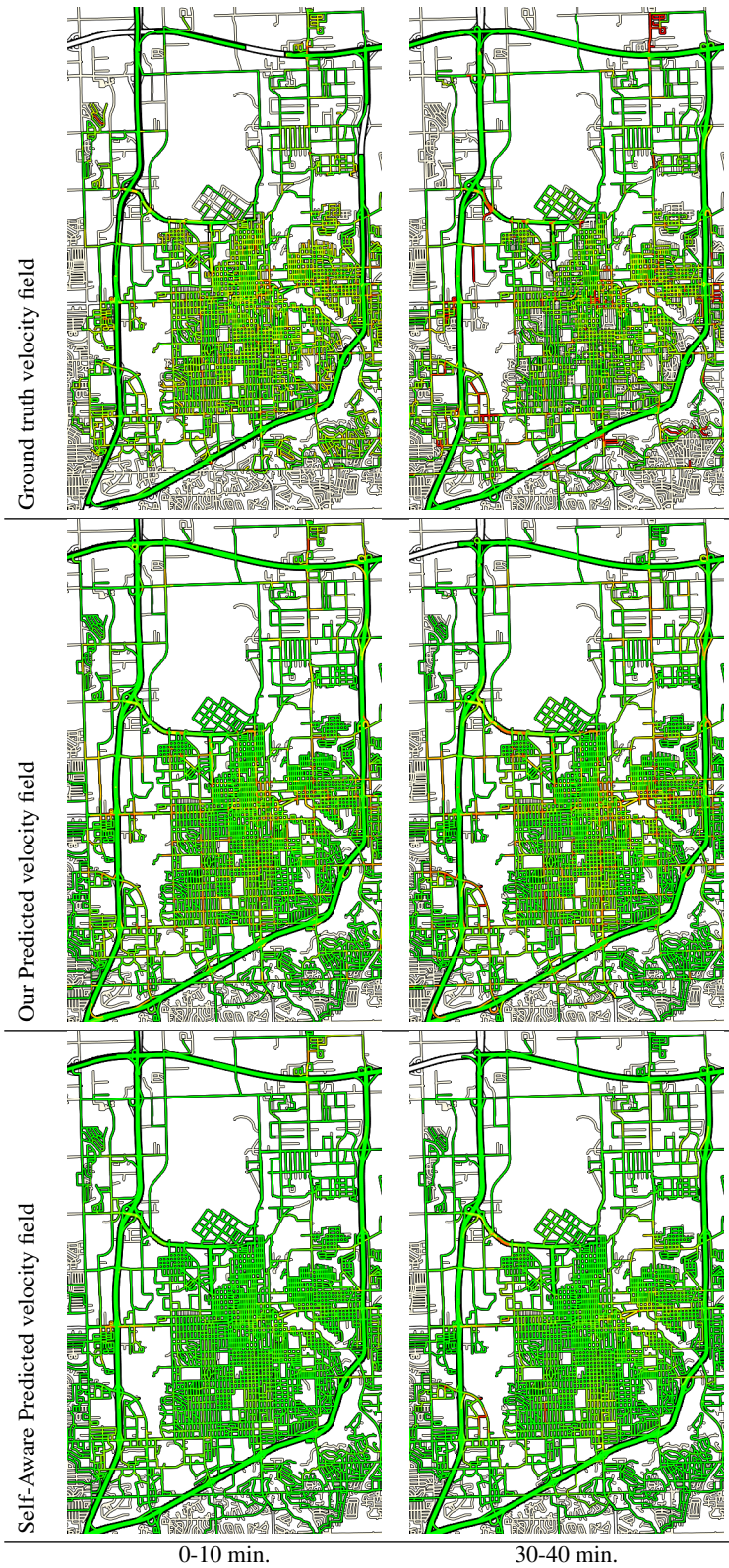
Figure 10: Each plot shows the mean velocity field over a ten minute time window, with a color ranging from red, 0 m/s, to green, 13 m/s. The top row is the ground truth; the middle row is the velocity field predicted solely by aggregating the routing requests of participating cars; the bottom row is the velocity field from using [27].
