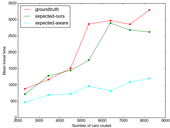
Figure 5: The mean travel time for the simulated ground truth (red), our method (green), and the self-aware routing algorithm (blue) for the MSMD scenario, described below. Our method can closely track the ground-truth travel time, while the self-aware algorithm systematically underestimates the actual travel time due to its inability to account for intersection delay.
